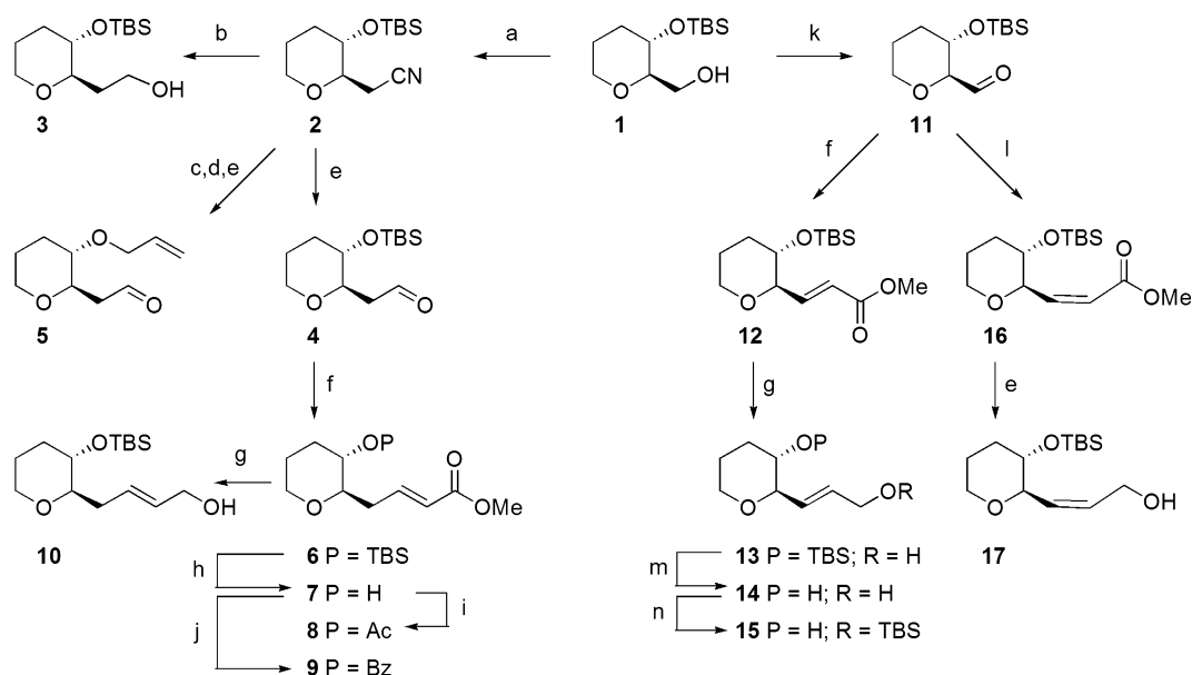
Scheme 1. Reagents and conditions: (a) i— \text{TsCl} , \text{Py} , \text{DMAP} , room temperature (rt); ii— \text{NaCN} , \text{DMSO} , 80^\circ\text{C} , 66%; (b) \text{DIBAL-H} , toluene, -78^\circ\text{C} , 14%; (c) \text{Bu}_4\text{NF} , \text{THF} , rt, 64%; (d) allyl bromide, \text{NaH} , \text{Bu}_4\text{NI} , \text{THF} , 0^\circ\text{C} to rt, 89%; (e) \text{DIBAL-H} , \text{THF} , 0^\circ\text{C} , for 4 92%, for 5 67%, for 17 76%; (f) (\text{MeO})_2\text{POCH}_2\text{CO}_2\text{Me} , \text{C}_6\text{H}_6 , \text{NaH} , rt, for 6 78%, for 12 88%; (g) \text{LiAlH}_4/\text{AlCl}_3 , \text{Et}_2\text{O} , -20^\circ\text{C} , for 10 93%, for 13 70%; (h) \text{Bu}_4\text{NF} , \text{HF} , rt, 52%; (i) \text{Ac}_2\text{O} , \text{DMAP} , \text{CH}_2\text{Cl}_2 , 86%; (j) \text{C}_6\text{H}_5\text{COCl} , \text{DMAP} , \text{CH}_2\text{Cl}_2 , 80%; (k) oxalyl chloride, \text{DMSO} , \text{Et}_3\text{N} , \text{CH}_2\text{Cl}_2 , -78^\circ\text{C} , 86%; (l) (\text{PhO})_2\text{POCH}_2\text{CO}_2\text{Me} , \text{THF} ; \text{NaH} , -78^\circ\text{C} , 86%; (m) \text{DOWEX 50W}\times 8 , \text{MeOH} , 68%; (n) \text{TBSCl} , imidazole, \text{CH}_2\text{Cl}_2 , rt, 75%.
